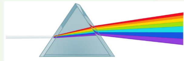
prism
