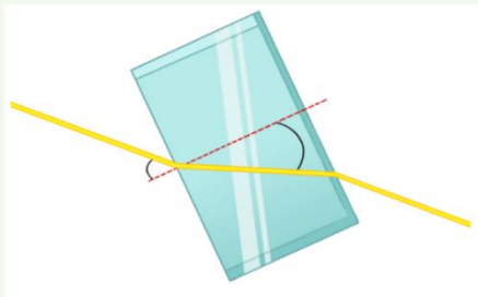
refraction
