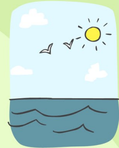
ocean
